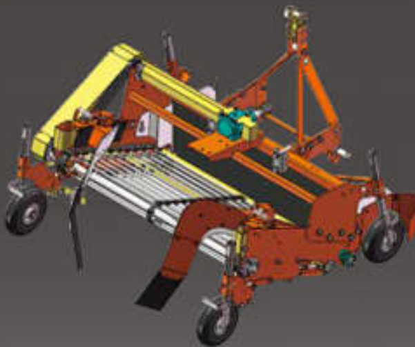
Square bar type
