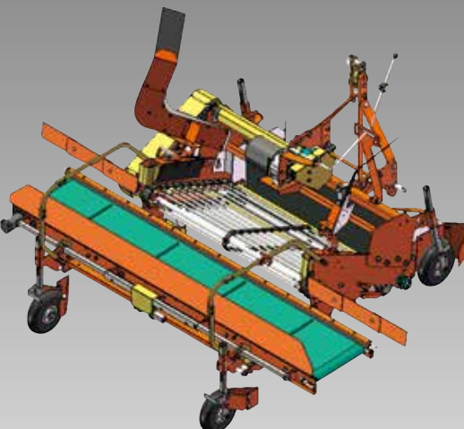
Square bar type
